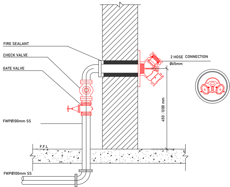
FIRE DEPARTMENT CONNECTION (FDC)
