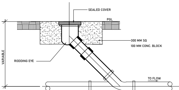
GROUND CLEANOUT
