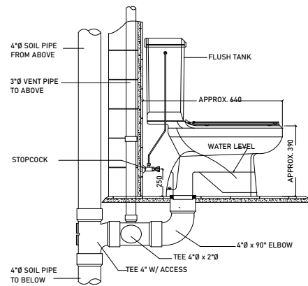
WATER CLOSET INSTALLATION DETAIL
