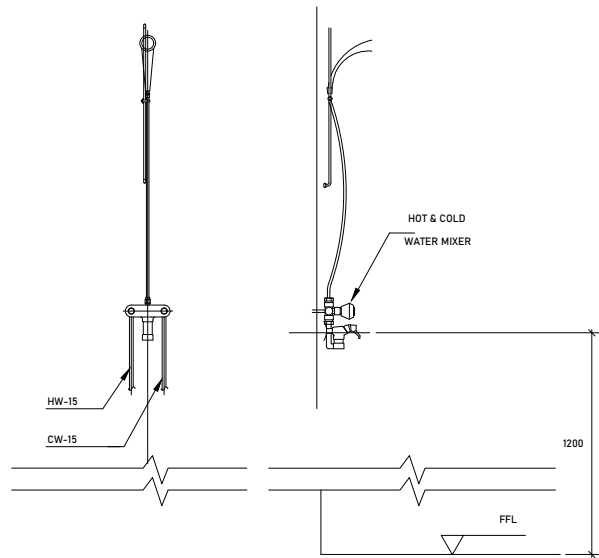
SHOWER
