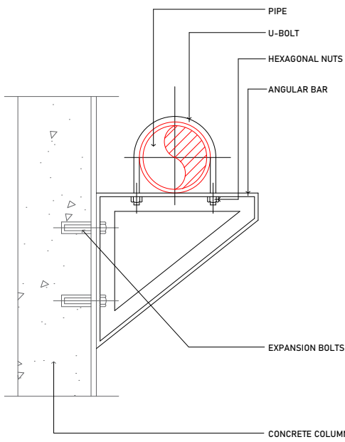
PIPE SWAY BRACE /BRACKET DETAIL
