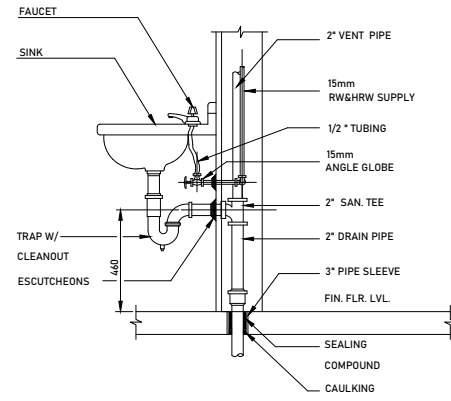
LAVATORY INSTALLATION DETAIL
