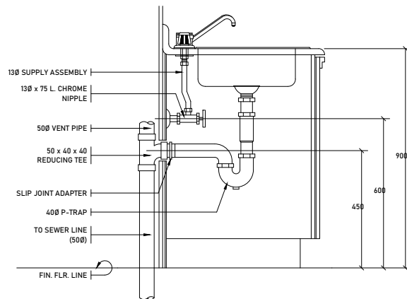
KITCHEN SINK INSTALLATION DETAIL
