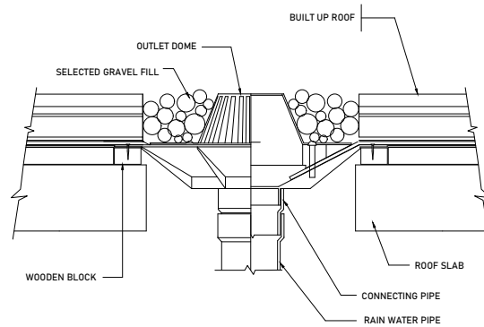
ROOF DRAIN DETAIL (DOME TYPE)
