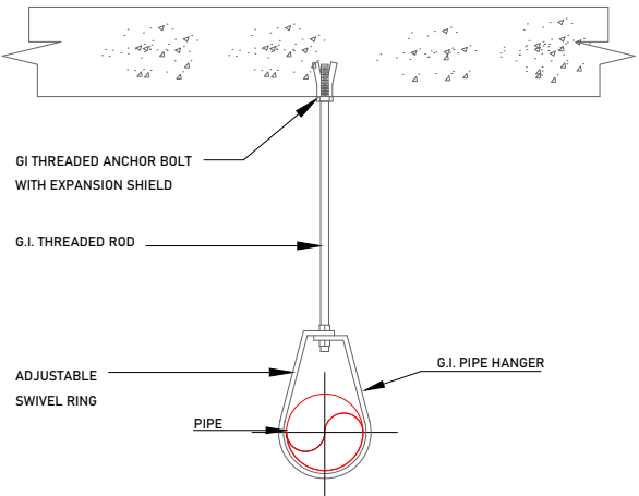
PIPE HANGER DETAIL
