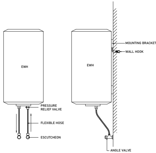
INSTALLATION DETAIL (VERTICAL) WATER HEATER
