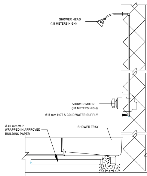
TYPICAL DETAIL OF SHOWER TRAY
