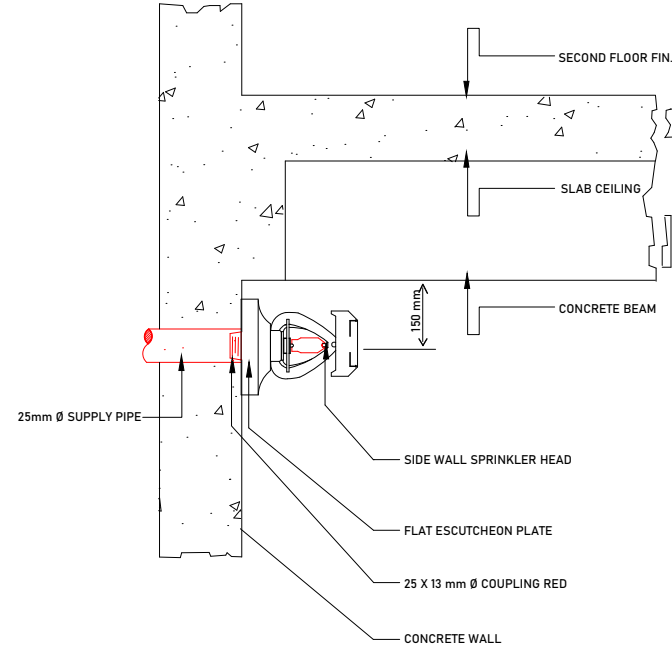
SIDEWALL SPRINKLER HEAD MOUNTING DETAIL
