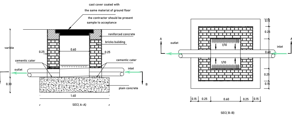
INSPECTION CHAMBER
