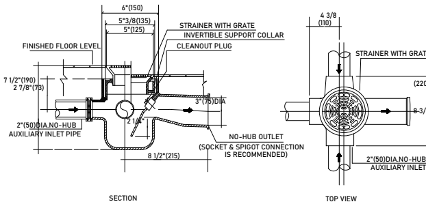
DETAIL OF FLOOR DRAIN
