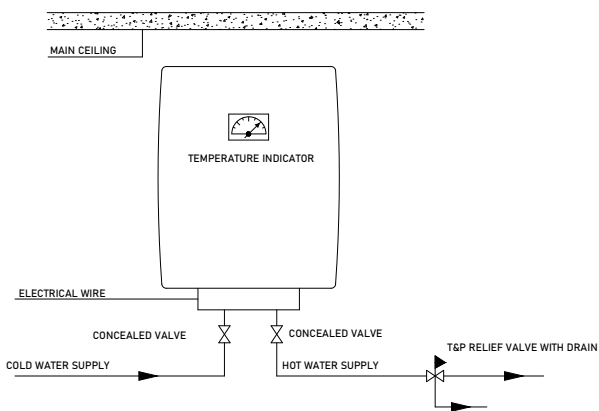
ELECTRIC WATER HEATER DETAIL (VERTICAL TYPE)
