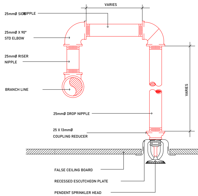
PENDENT SPRINKLER HEAD CONNECTION DETAIL
