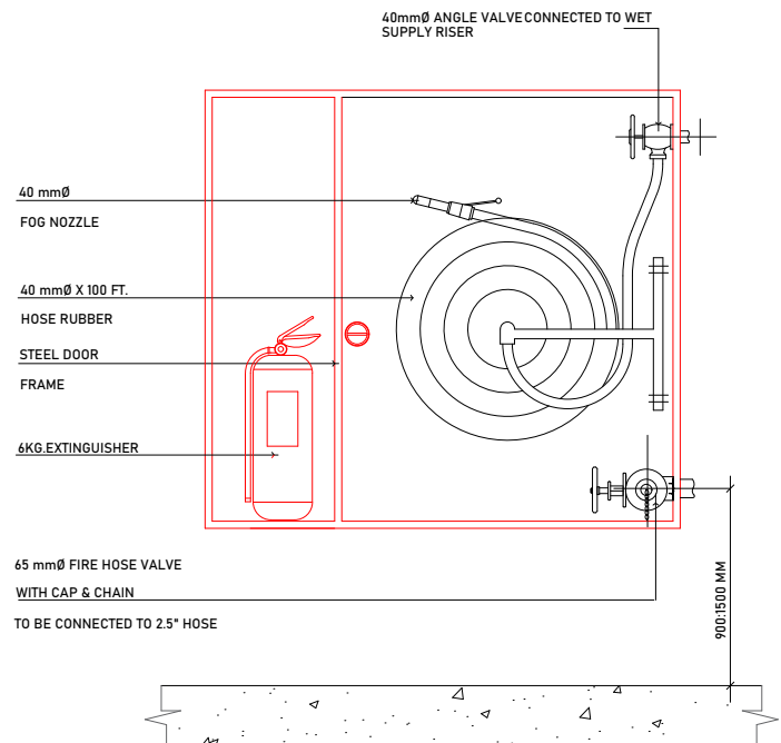
FIRE HOSE VALVE AND FIRE HOSE CABINET DETAIL
